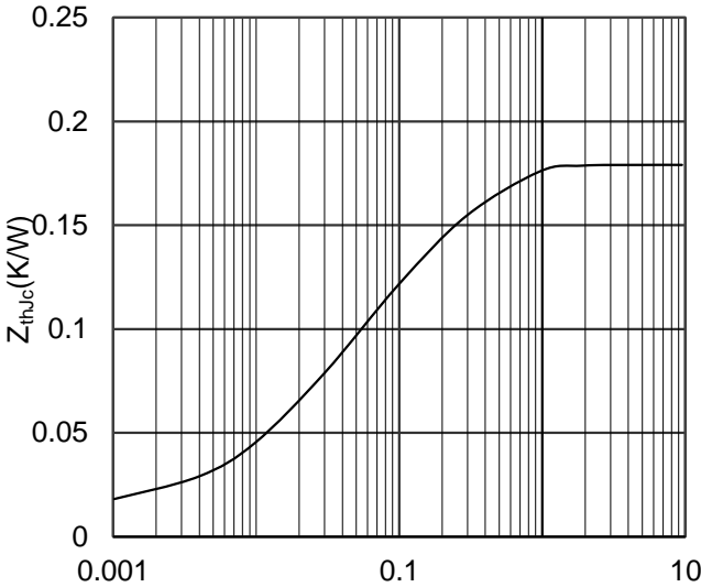
Rectangular Pulse Duration (s) Figure 5. Transient Thermal Impedance
